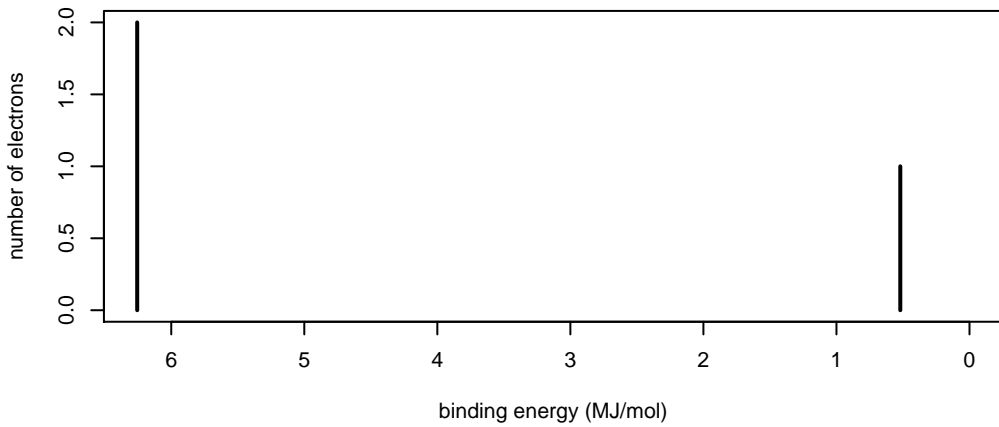
lithium
