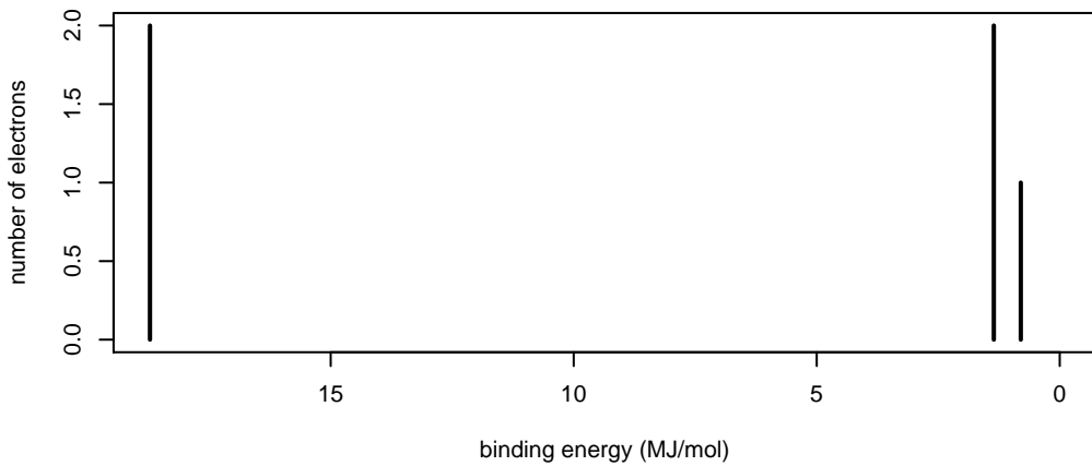
boron
