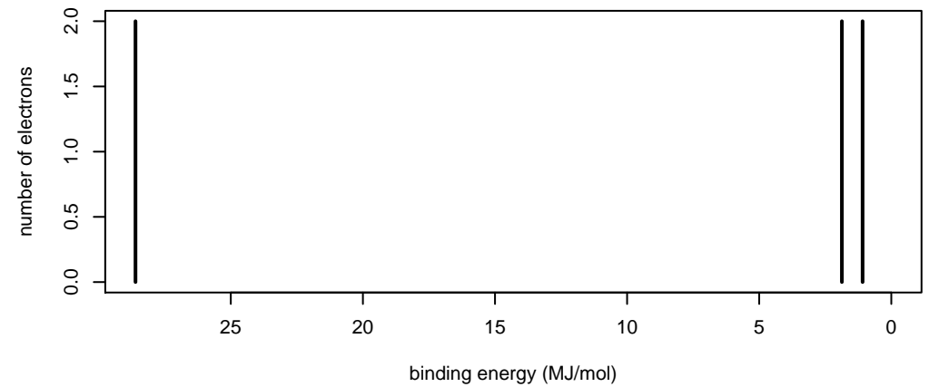
carbon
