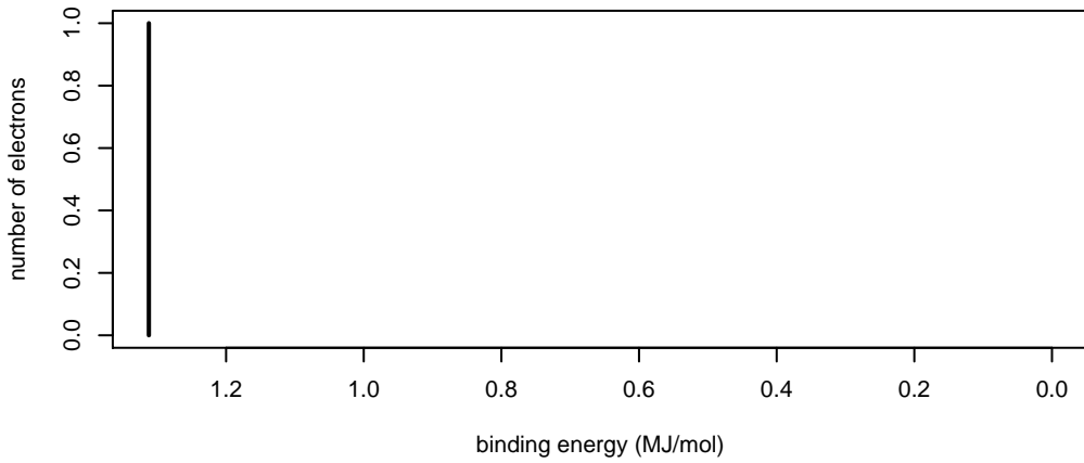
hydrogen
