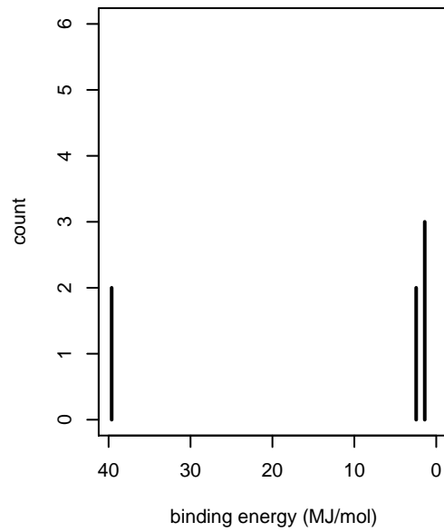
nitrogen
