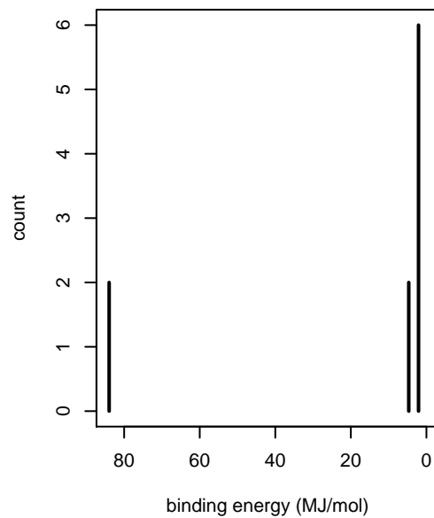
neon
