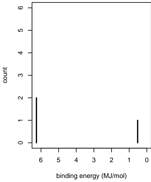
lithium
