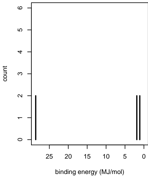
carbon
