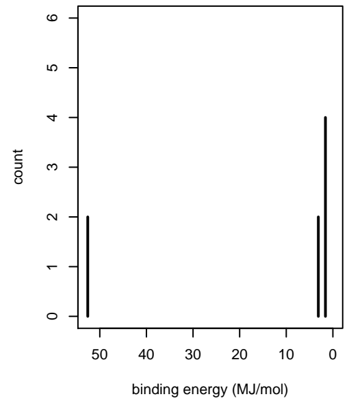
oxygen
