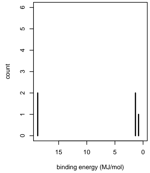
boron
