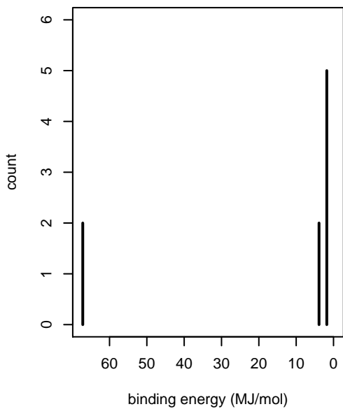
fluorine
