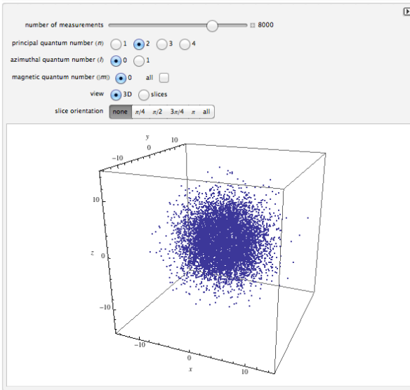
2s orbital
