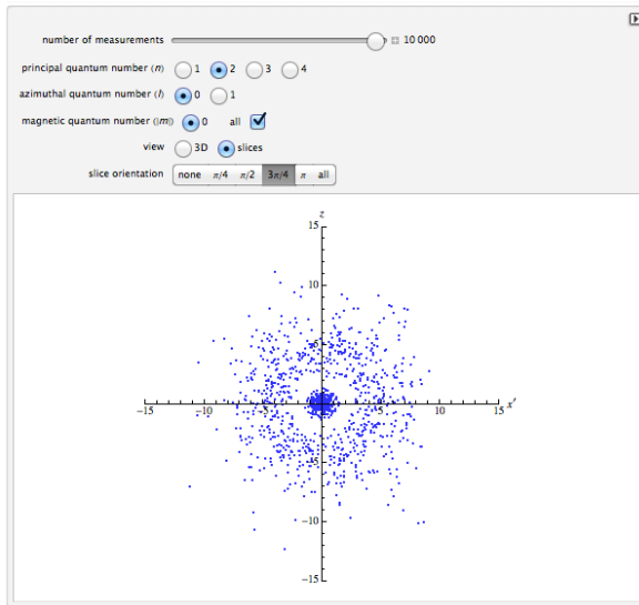
2s orbital
