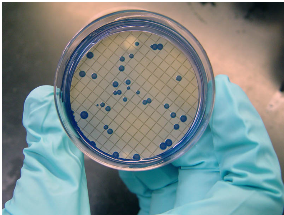
Figure 3.1 Colonies of fecal coliform bacteria from a water supply. Source: Susan Boyer ( www.ars.usda.gov ).
